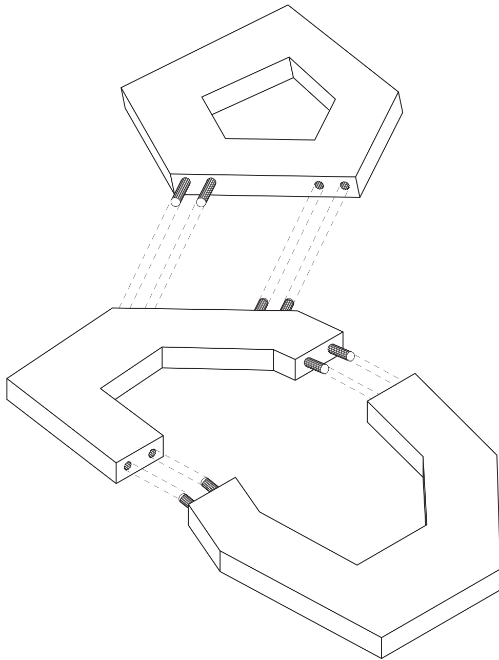
DOWEL JOINT ASSEMBLY SCALE // 1:4
