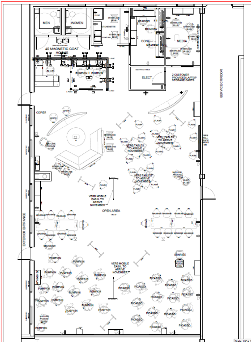
PLAN VIEW 1/4"=1'-0"
