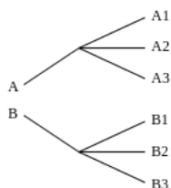
Figure 1: Illustration of a Possibility Tree, Source: Wikipedia
