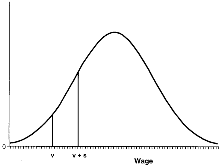
Fig. 1. Wage distribution.
