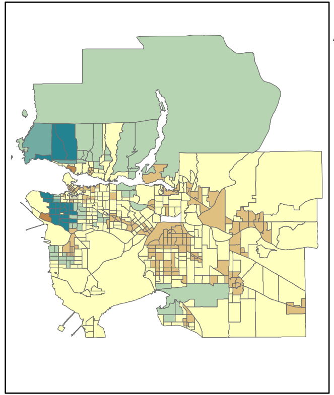
Standard Deviation
