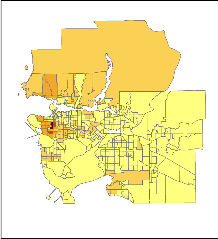
Equal Interval
