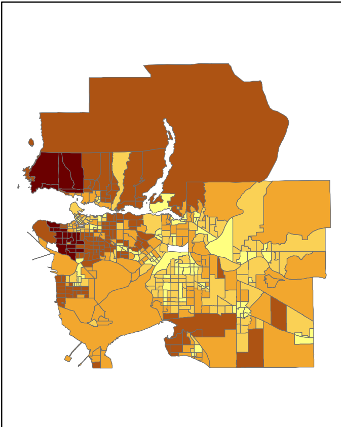
Natural Breaks
