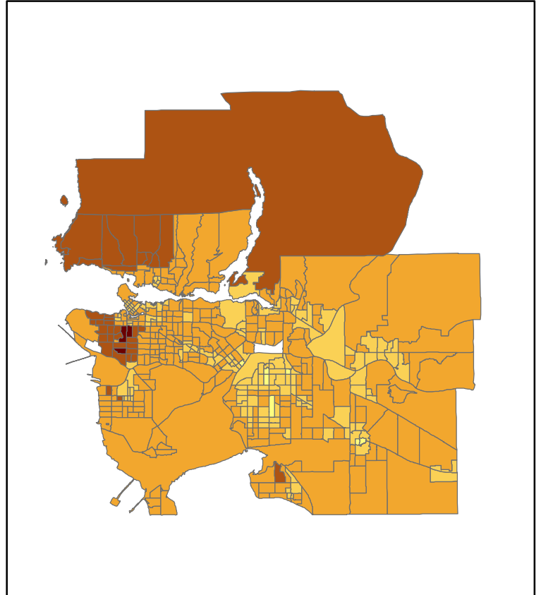
Manual Break
