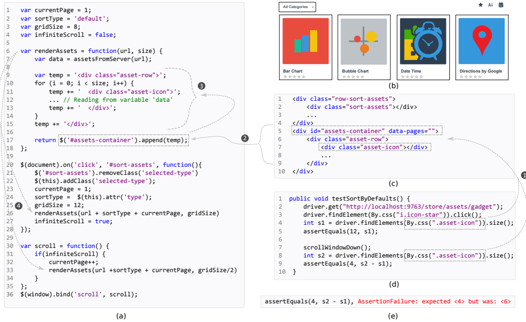
Fig. 3: Test assertion understanding example (a) JavaScript code, (b) Portion of DOM-based UI, (c) Partial DOM, (d) DOM-based (Selenium) test case, (e) Test case assertion failure. The dotted lines show the links between the different entities that must be inferred.
