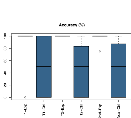
Fig. 21: Box plots of task completion accuracy data per task and in total for the control (blue) and experimental (cream) groups (higher values are desired). [Study 3]
