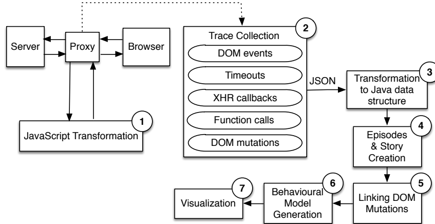
Fig. 4: A processing overview of our approach.
