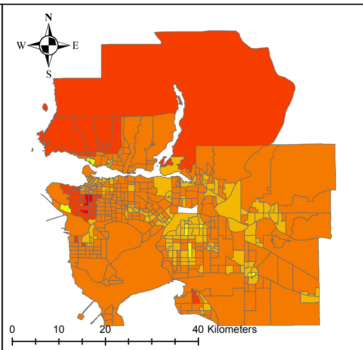
Equal Interval Classification
