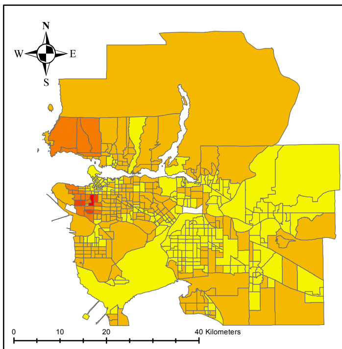
Manual Breaks Classification
