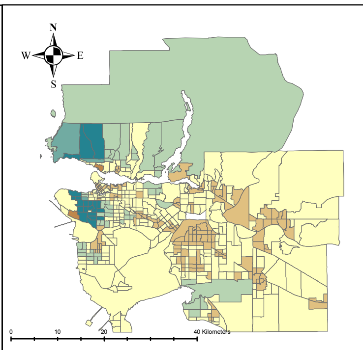
Standard Deviation Classification
