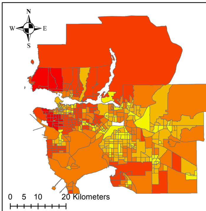
Natural Breaks Classification
