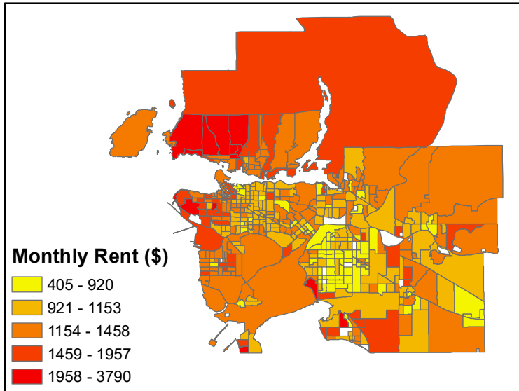
Natural Breaks
